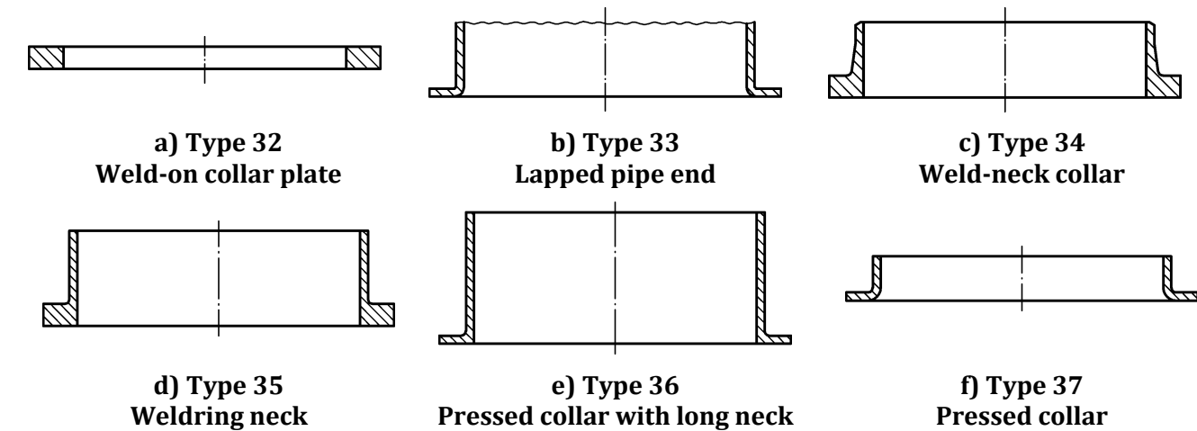
Figure 2 — Collars types 32 to 37
